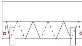
Fig. 6 Heating cable arrangement on a horizontal tank
