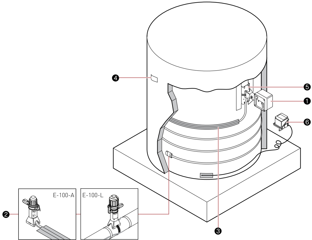
Fig. 8 Tank-tracing system connection kits and accessories
